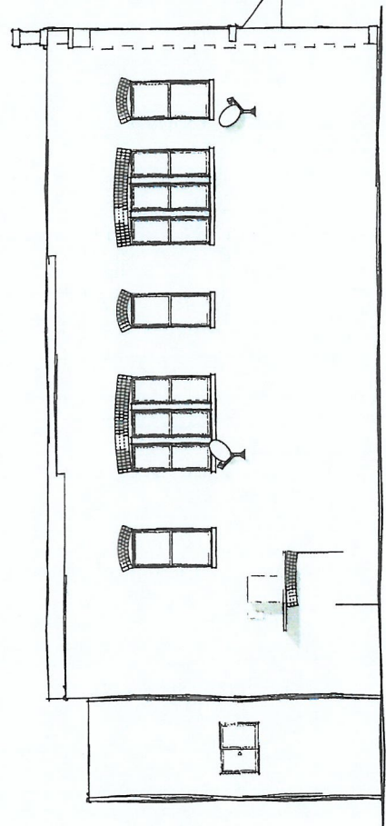
EXISTING SOUTH ELEVATION AS SHOWN 1/4" = 1'-0"
